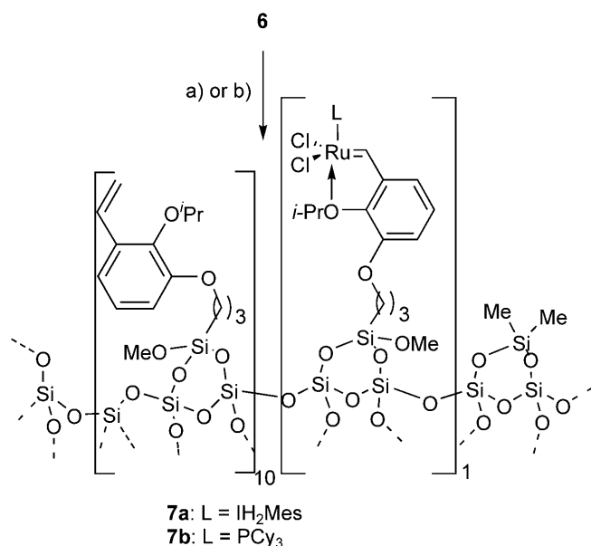
Scheme 2. a) Grubbs–Herrmann catalyst (0.1 equiv.), \text{CuCl} (0.1 equiv.), \text{CH}_2\text{Cl}_2 , \text{N}_2 , 45^\circ\text{C} , 3 h, loading 33.6\ \mu\text{mol/g} ; b) Grubbs catalyst (0.1 equiv.), \text{CH}_2\text{Cl}_2 , \text{N}_2 , 45^\circ\text{C} , 3 h, loading 17.4\ \mu\text{mol/g}
